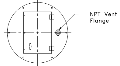
Hinged and Lockable Cover
