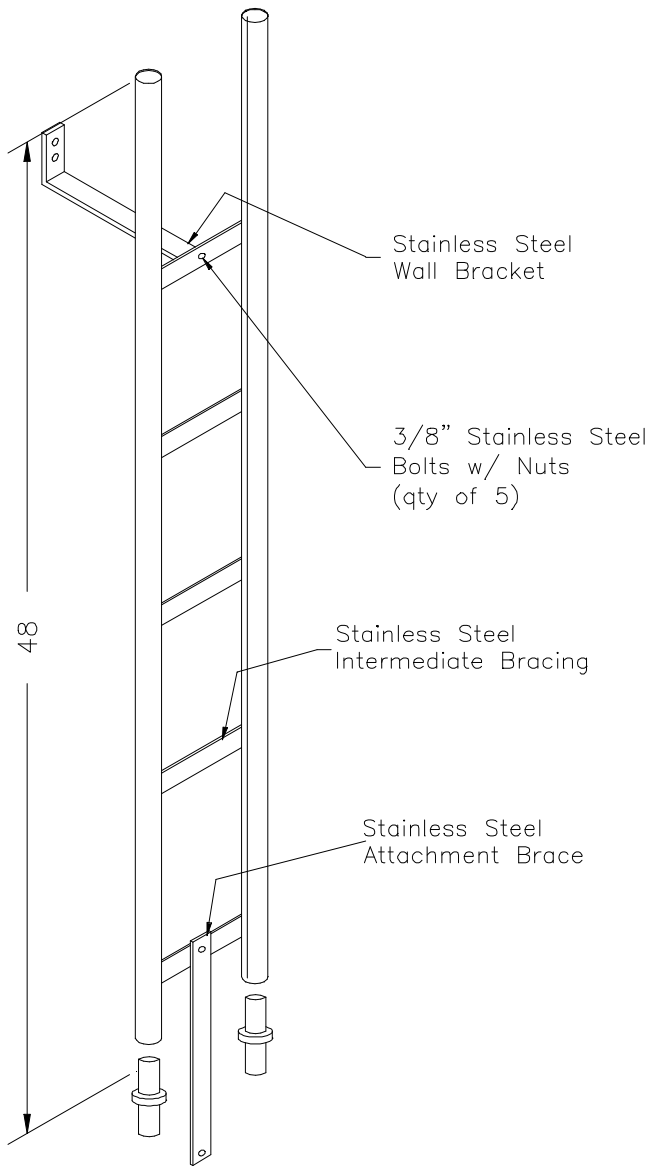
Part #: SGR-48 Ext.
